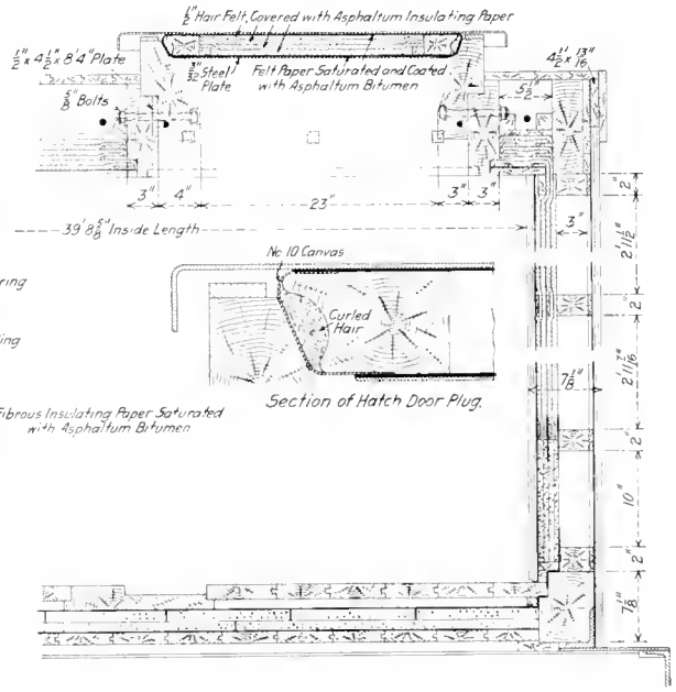
Sections Through the Ice Hatch Showing the Insulation on the Sides, Ends and Floor of the Car
